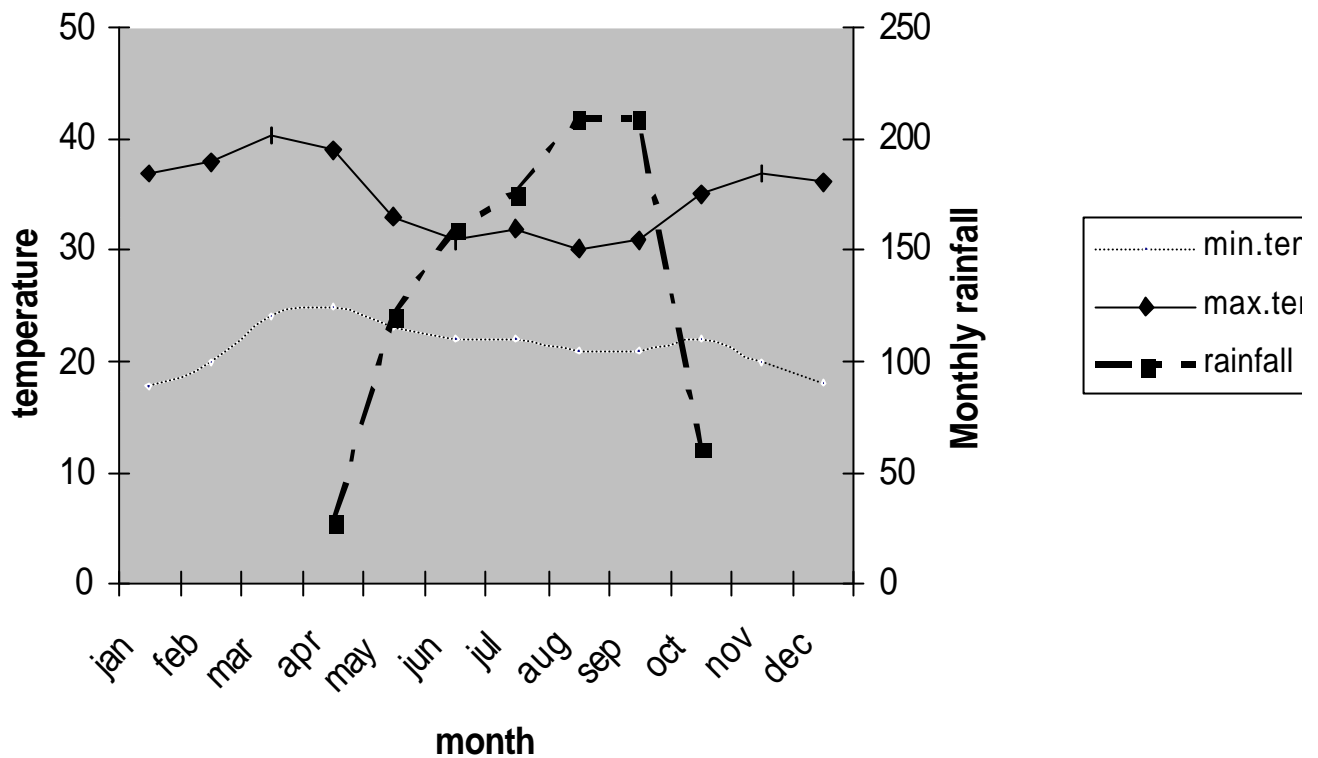
Fig 5.1 Comparison for seasonal Rainfall and Temperature at Garoua (mean of 34 years (1950 -1984))
