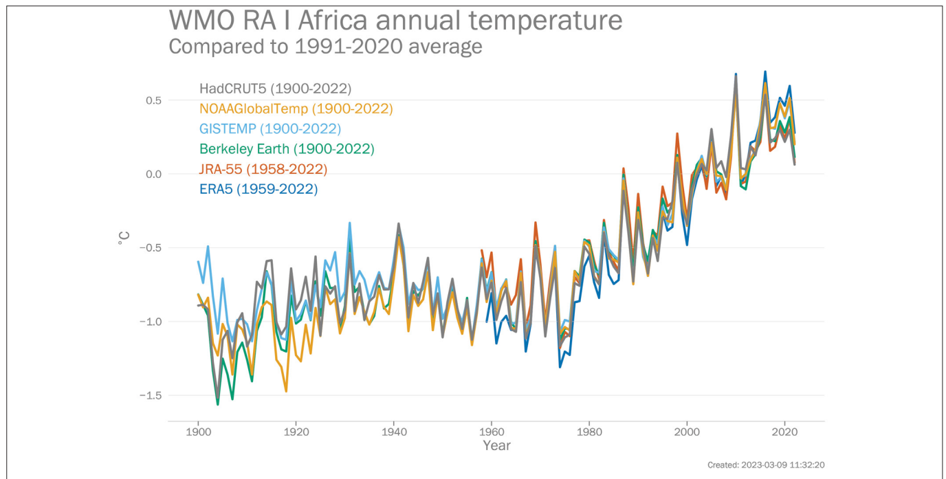
Figure 2. Temperature difference in °C with respect to the 1991–2020 climatological period for Africa (WMO Regional Association I) from 1900 to 2022, based on six data sets, including observational data sets (HadCRUT5 [black], NOAA GlobalTemp [yellow], GISTEMP [light blue], and Berkeley Earth [green]) and reanalyses (JRA-55 [orange] and ERA5 [dark blue])
